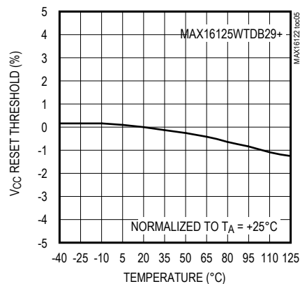
V_{CC} RESET THRESHOLD vs. TEMPERATURE
